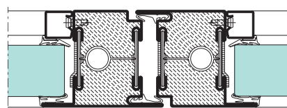
Janisol C4 EI60/EI90
